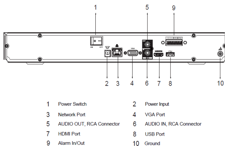
Figura 1 - Painel iNVD 3032
